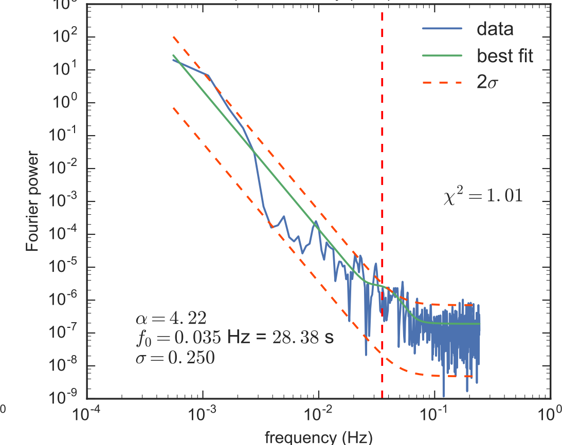
Power Spectral Density (PSD) - Model 1
