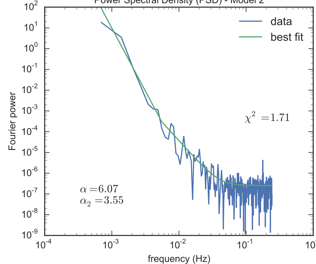
Power Spectral Density (PSD) - Model 2
