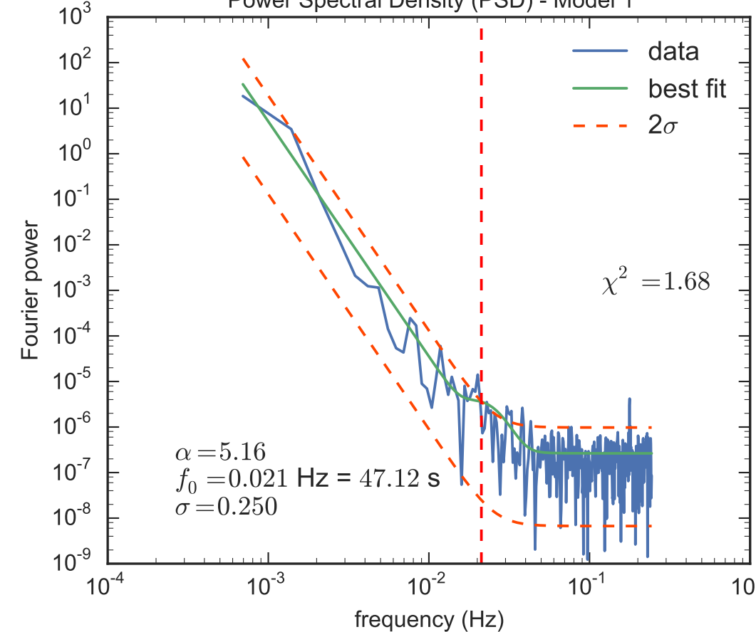
Power Spectral Density (PSD) - Model 1
