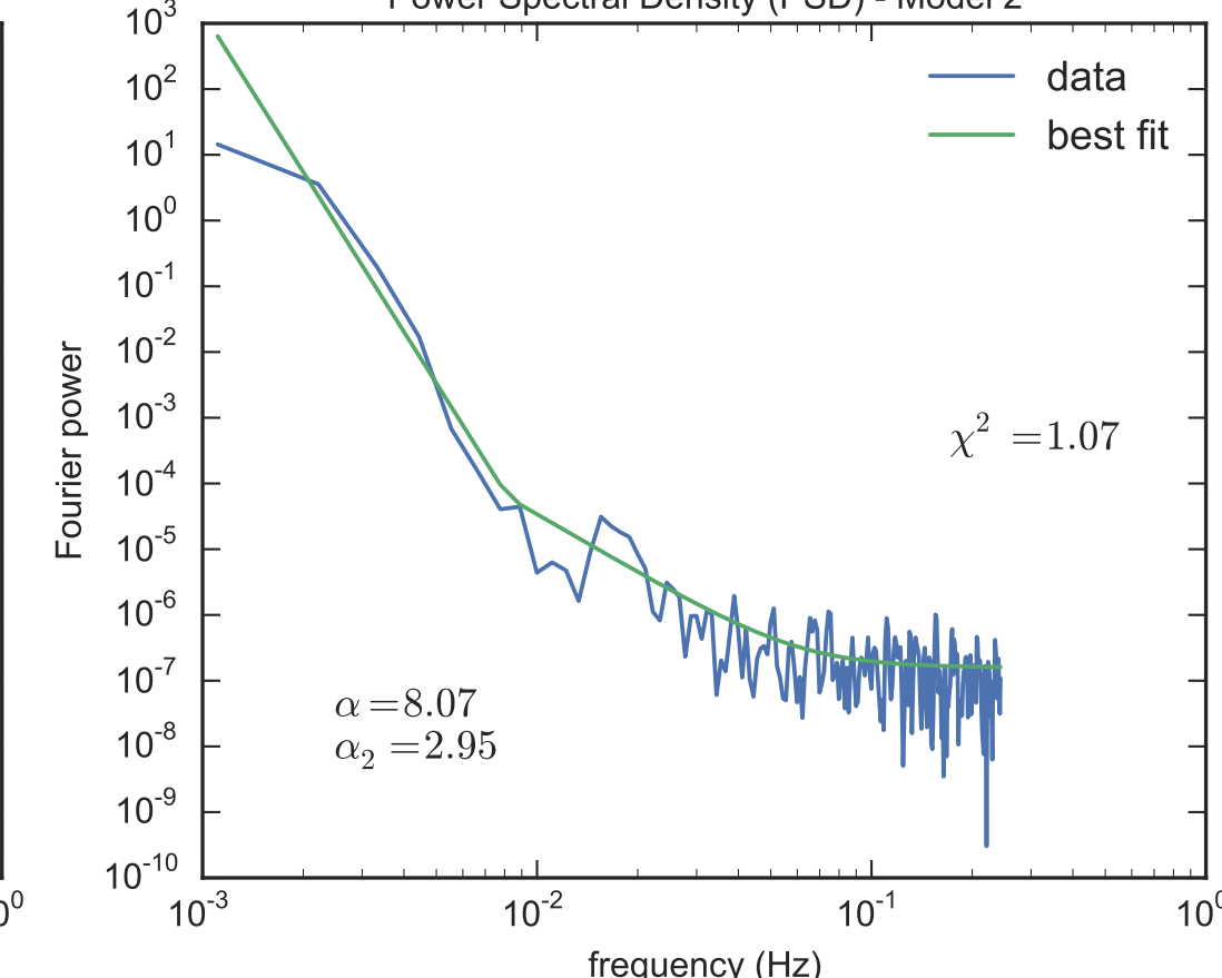
Power Spectral Density (PSD) - Model 2
