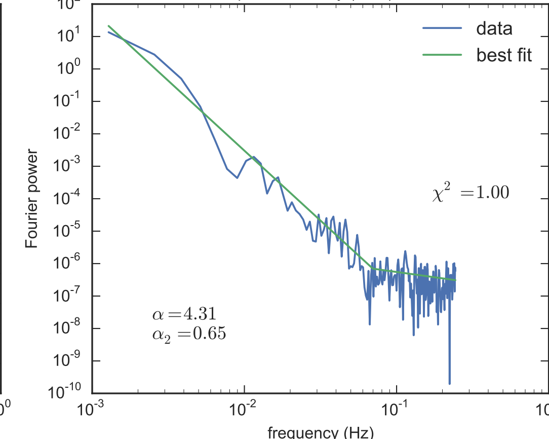
Power Spectral Density (PSD) - Model 2
